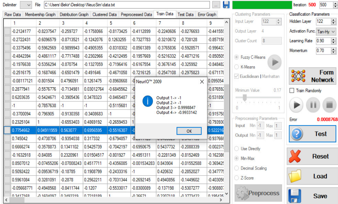
FIGURE 3: Graphical Interfaces of proposed FCNN.
